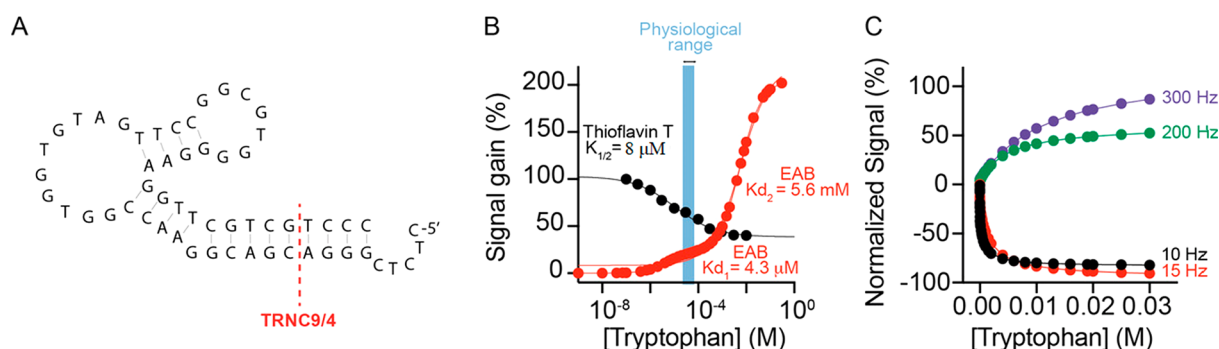
Figure 4. When we adapt (A) the TRNC9/4 truncation of our tryptophan-binding aptamer into an EAB sensor its binding midpoint (B) moves to 700-fold higher concentrations than that seen when binding is monitored in solution using thioflavin T fluorescence. Noticing a small transition in the EAB binding curve at low target concentrations we hypothesized that this discrepancy occurs because the full-length aptamer binds two copies of its target, one at an affinity of \sim 1 \mu\text{M} and a second with affinity of several millimolar. Consistent with this, a two-site model fits the EAB data quite well (solid line; R^2 = 0.998 ), producing a small-amplitude event with a binding midpoint of 4.3 \pm 0.7 \mu\text{M} and a much larger amplitude event with a binding midpoint to approximately 5 mM. Note: the EAB data shown here are reported as % change in KDM, with the KDM being derived from interrogations at square-wave frequencies of 15 and 300 Hz. (C) A study of the square-wave frequency dependence of the EAB sensor response curves provides further evidence in favor of this two-site hypothesis. Specifically, whereas the higher-affinity binding event is readily apparent at lower square-wave frequencies, at higher frequencies the lower-affinity binding event dominates the data (see Table S1 for the two-site-model fit parameters). Such strong frequency dependence to the binding curves is not typically seen for single-site aptamers. 21
