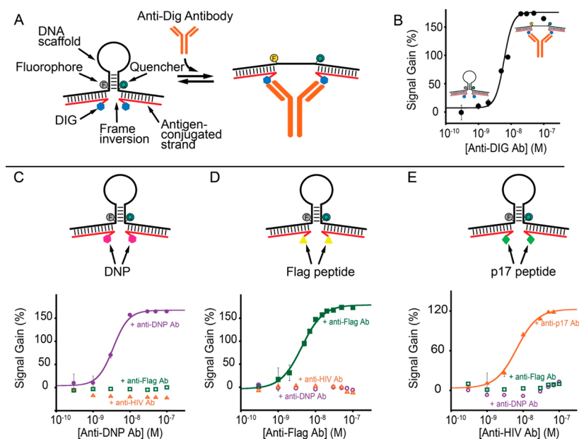
Figure 1. DNA-based structure switching probes for optical antibody detection. (A) The optical antibody-switch platform is designed to adopt a two-tailed stem–loop conformation in the absence of the target antibody. The two single-stranded tails act as an anchoring strand for DNA complementary sequences that are conjugated at one end with an appropriate recognition element (i.e., digoxigenin antigen) for the target antibody (anti-digoxigenin antibody). The binding of one copy of a target antibody to the two recognition elements causes a conformational change resulting in the opening of the stem–loop conformation and in an increase in the fluorescence signal intensity. (B) The antibody-switch sensor detects anti-digoxigenin antibodies at low nanomolar concentrations. (C–E) The modular nature of the platform allows the detection of different targets by changing the recognition element [C, dinitrophenol (DNP); D, eight-residue FLAG peptide; E, 13-residue epitope excised from HIV protein p17] in a nanomolar concentration range, without any significant cross-reactivity with the other nonspecific targets. Reproduced from A Modular, DNA-Based Beacon for Single-Step Fluorescence Detection of Antibodies and Other Proteins. Ranallo, S.; Rossetti, M.; Plaxco, K. W.; Vallée-Bélisle, A.; Ricci, F. Angew. Chem., Int. Ed. 2015, Vol. 54, Issue 45 (ref 89). Copyright 2015 Wiley.
